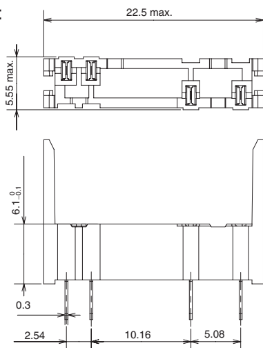
Connecting Socket P6DS-04P
